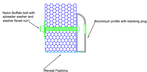
'A' Frame Head Detail
